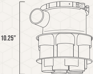
C5 Valve
